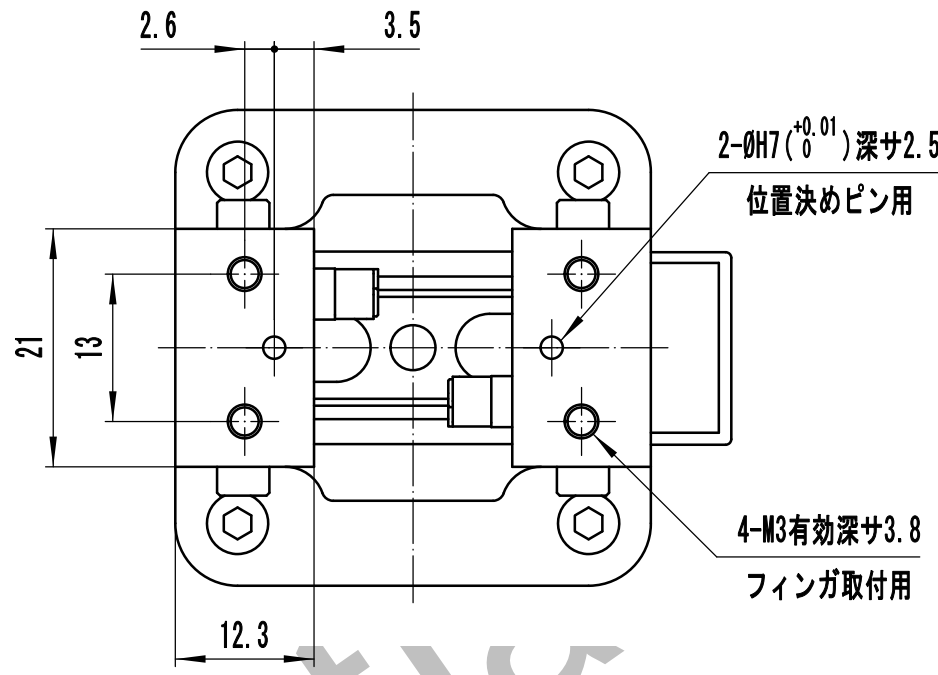
矢視A(1.5:1)
